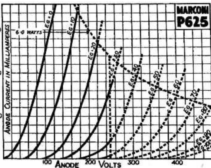
Anode Volts, Anode Current Curve for P 625.
